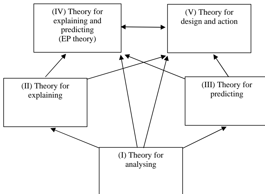
Figure 1: Interrelationships among theory types
